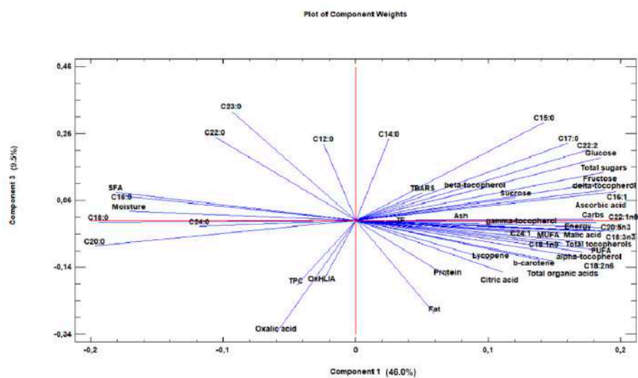
Figure 7. The loading plot of principal components 1 and 3 for processing tomato fruit.
